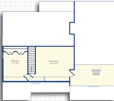
Optional Bedroom 5 with Optional Finished Bonus Room Elevation A & B - Also available with open rail staircase to the bonus room.
