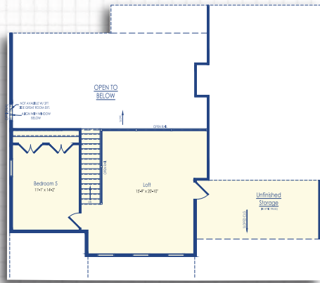
Optional Loft with Bedroom 5 Elevation D
