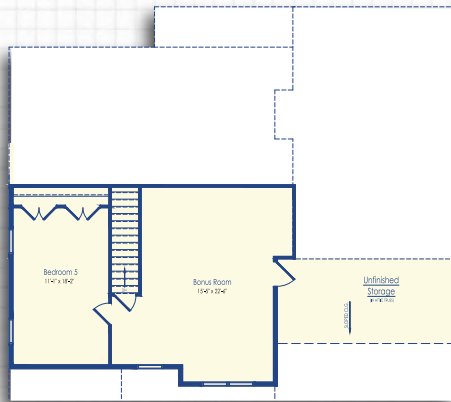
Optional Bedroom 5 with Optional Finished Bonus Room Elevation F- Also available with open rail staircase to the bonus room.
