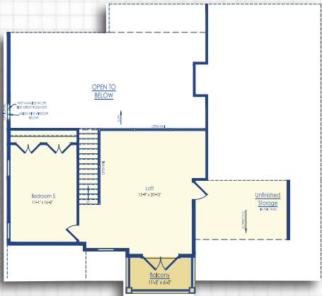
Optional Loft with Bedroom 5 Elevation E
