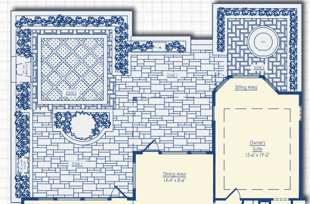
Optional Courtyard with Spa Extension, Owner's Sitting Area, and Covered Porch I
