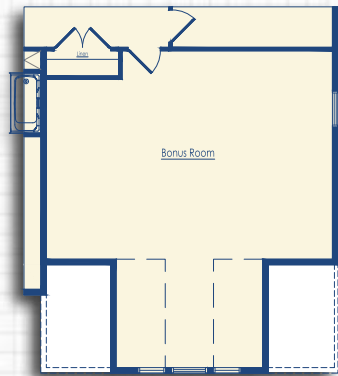
Optional Bonus Room with 4' Garage Extension Craftsman Style
