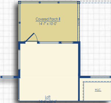
Optional Covered Porch II
