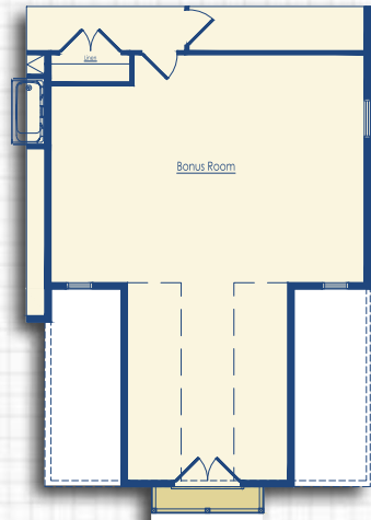
Optional Bonus Room with 3-Car Side Load Garage Schell Style C
