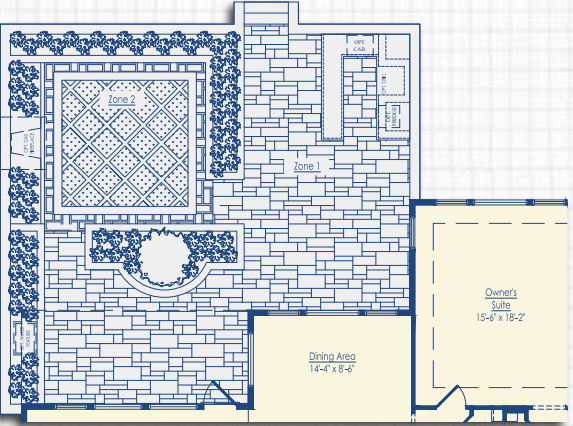
Optional Courtyard with Deck IV Above and Outdoor Kitchen
