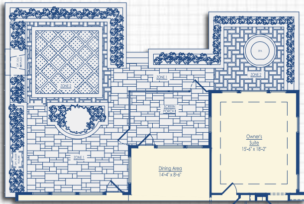
Optional Courtyard with Spa Extension and Screen Porch I
