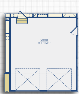
Optional 4' Garage Ext. Schell Style B
