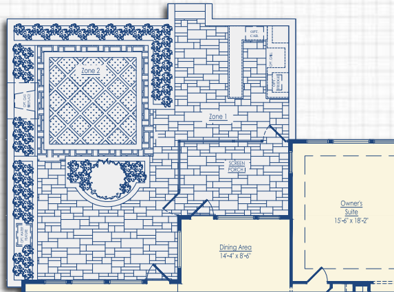
Optional Courtyard with Screen Porch I and Outdoor Kitchen
