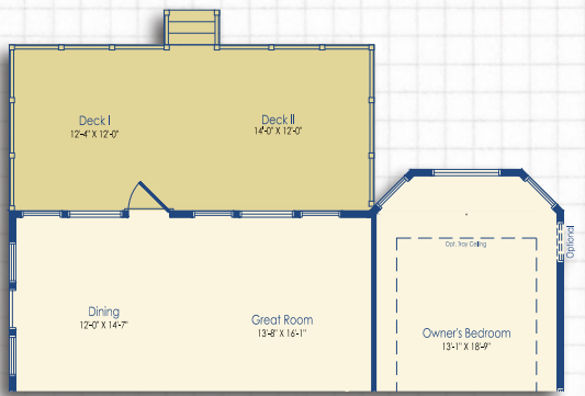
Optional Deck I and Deck II with Optional Luxury Owner's Bath I/II and Optional 2 Ft. Rear Extension
