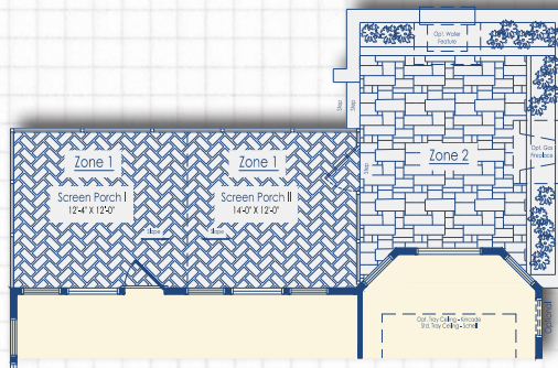
Optional Courtyard with Optional Screen Porch I and Screen Porch II with Optional Luxury Owner's Bath I/II and Optional 2 Ft. Rear Extension
