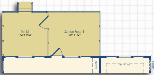
Optional Optional Deck I with Screen Porch II
