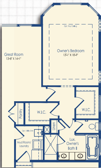
Optional Luxury Owner's Suite II
