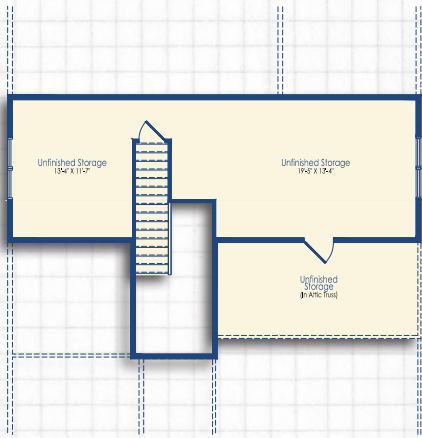
Optional Unfinished Storage Elevation A
