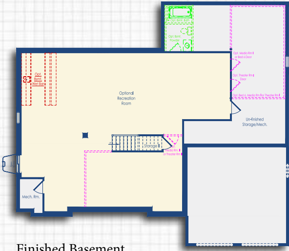
Finished Basement *Shown with Elevation A
