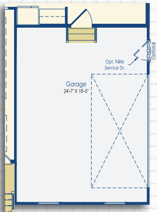
Optional Side Load Garage with 4' Garage Extension Schell Style A, Craftsman Style and Beach Style
