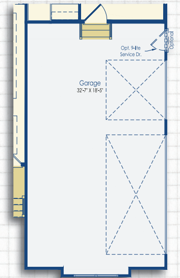
Optional 3-Car Side Load Garage Schell Style B
