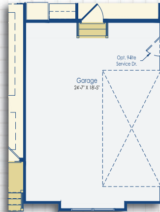
Optional Side Load Garage Schell Style B
