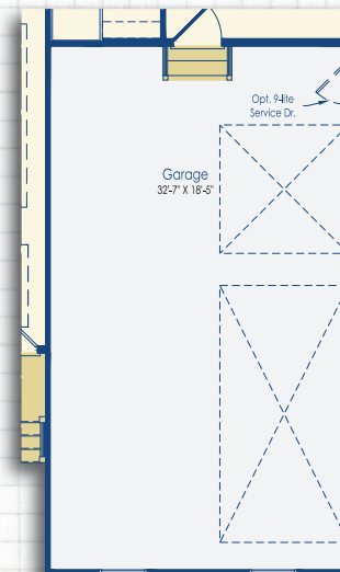
Optional 3-Car Side Load Garage Schell Style A, Craftsman Style and Beach Style
