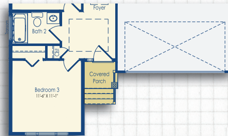
Optional Craftsman Style
