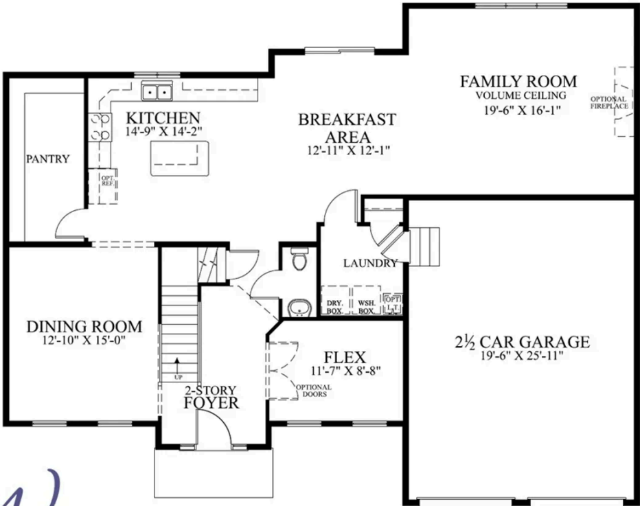
First Floor (Traditional Elevation)
