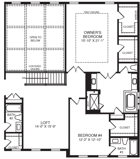
OPT. FOUR BEDROOM W/ LOFT
