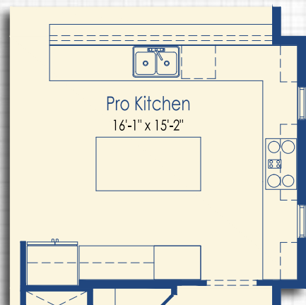
Optional Extended Professional Kitchen Second Floor *Shown with optional island
