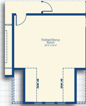
Second Floor Plan with Optional 4' Extension Craftsman Elevation
