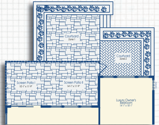
Optional Courtyard with Screen Patio I & II and Luxury Owner's Suite
