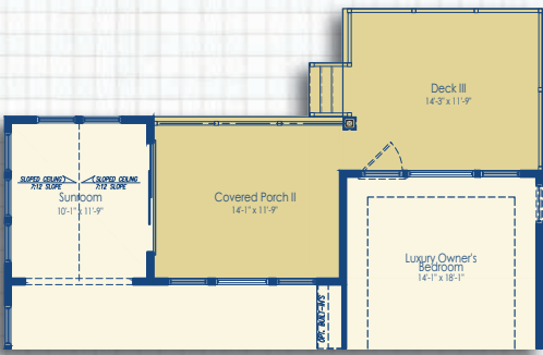
Optional Sunroom with Covered Porch II, Deck III, & Luxury Owner's Suite
