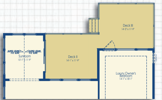
Optional Sunroom with Deck II & III and Luxury Owner's Suite
