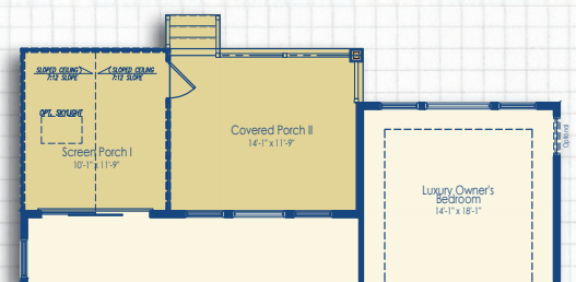
Optional Screen Porch I & Covered Porch II with Luxury Owner's Suite
