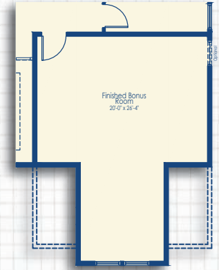
Second Floor Plan with Optional 4' Extension Modern Farmhouse Elevation
