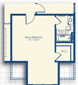
Bonus Bedroom with Bath Modern Farmhouse Elevation
