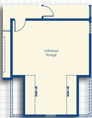
Second Floor Plan with Optional 4' Extension Elevation A
