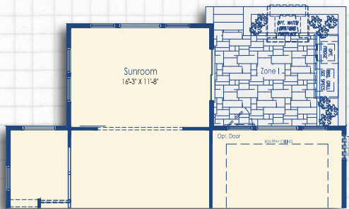
Optional Courtyard with Optional Sunroom
