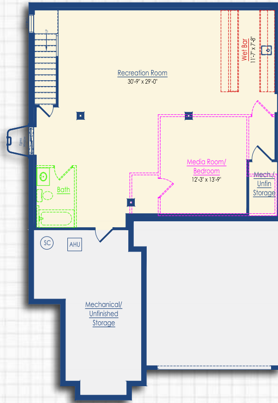
Finished Basement
