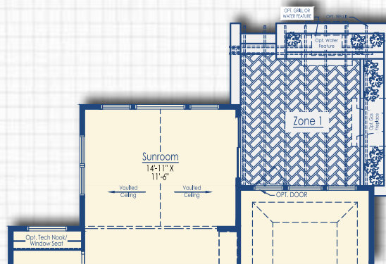
Optional Sunroom & Courtyard I with 4' Owner's Suite Extension
