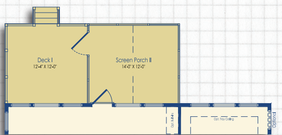
Optional Deck I with Optional Screen Porch II
