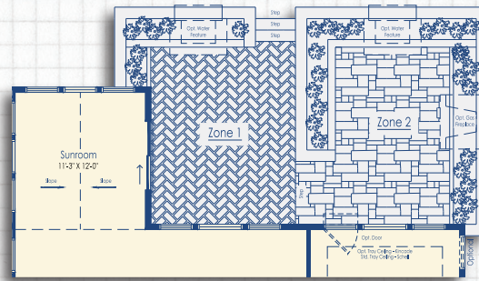
Optional Courtyard with Sunroom
