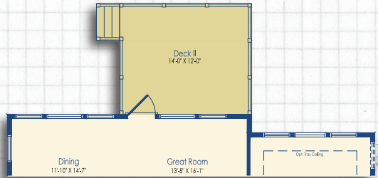
Optional Deck I with Optional 2 Ft. Rear Extension
