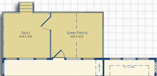
Optional Screen Porch II and Optional Deck I with Optional Luxury Owner's Bath I/II and Optional 2 Ft. Rear Extension
