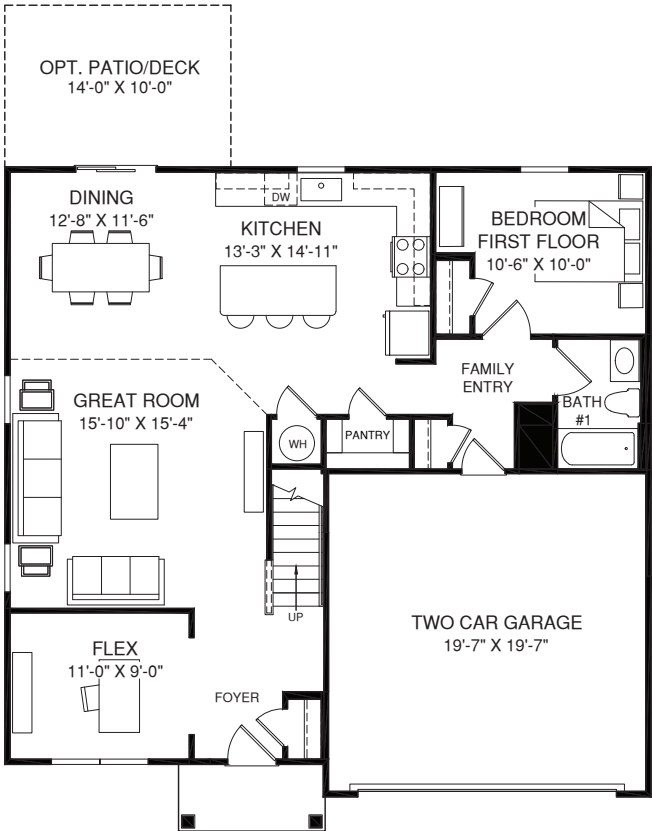
MAIN LEVEL
