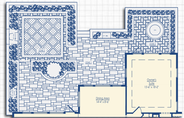
Optional Courtyard with Spa Extension
