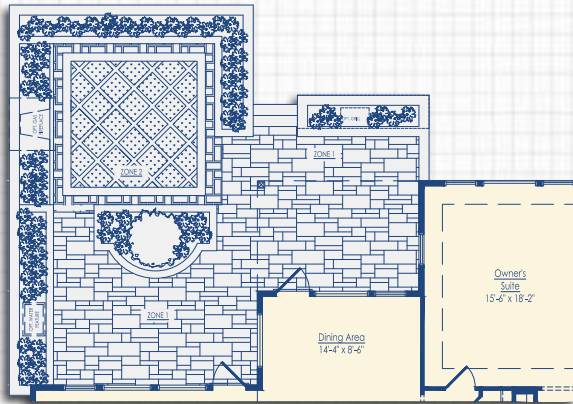
Optional Courtyard with Covered Porch I
