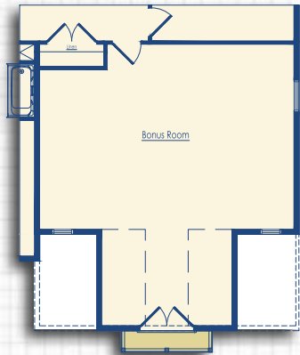
Optional Bonus Room with 4' Garage Extension Schell Style C
