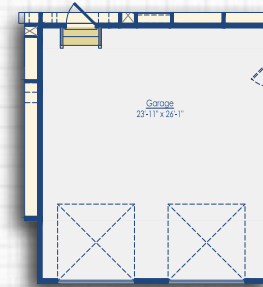
Optional 4' Garage Ext. Craftsman Style
