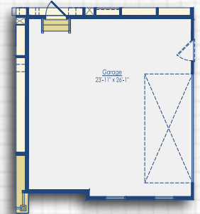
Optional Side Load Garage with 4' Garage Ext. Southern Style
