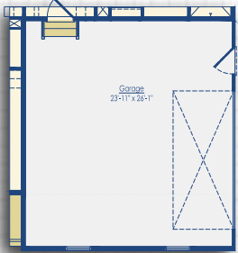
Optional Side Load Garage with 4' Garage Ext. Schell Style A
