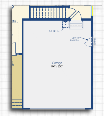
Optional 4' Garage with Basement Stairs Elevation B & D
