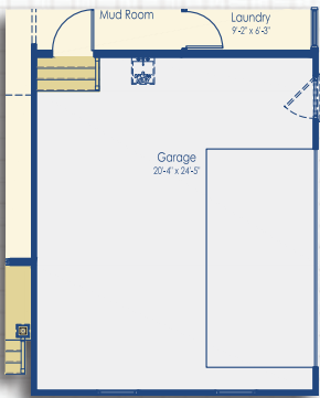
Optional Side Load Garage with 4' Extension Southern Elevation
