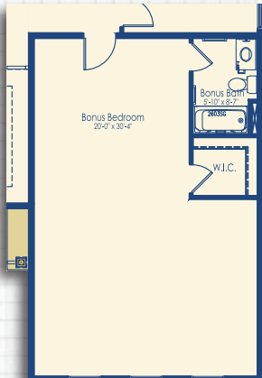
Bonus Bedroom with Bath & 4' Garage Extension Southern Elevation
