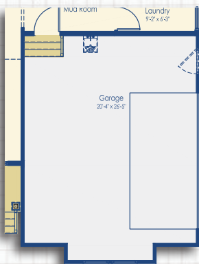
Optional Side Load Garage with 4' Extension Modern Farmhouse Elevation
