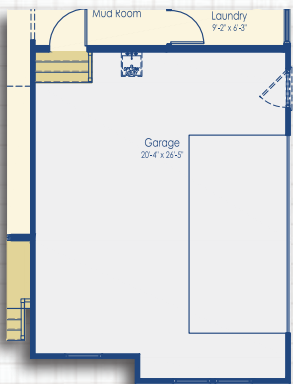
Optional Side Load Garage with 4' Extension Elevation B
