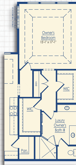
Optional Luxury Owner's Suite III
