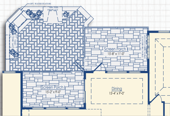
Optional Courtyard with Screen Porch I & II
