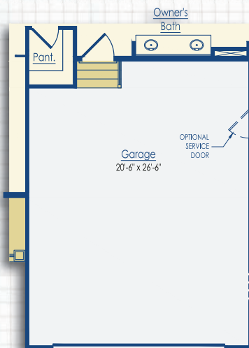
Optional 4' Garage Extension Elevation A/B/C/D
