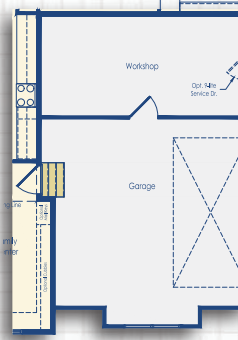
Optional Side Load Garage with 9' Garage Extension and Optional Workshop Schell Style A
