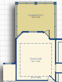
Optional Covered Porch II with Owner's Suite Bay Window *Screen Porch I Below
