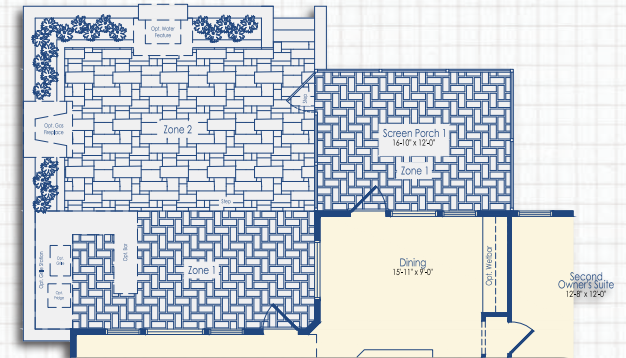
Optional Courtyard with Screen Porch I
