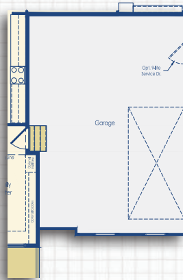
Optional Side Load with 9' Garage Extension Southern Style
