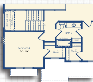
Optional Bedroom 4 Schell Style C
