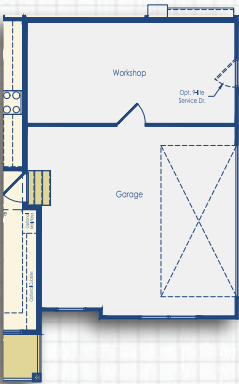
Optional Side Load Garage with 9' Garage Extension and Optional Workshop Schell Style C
