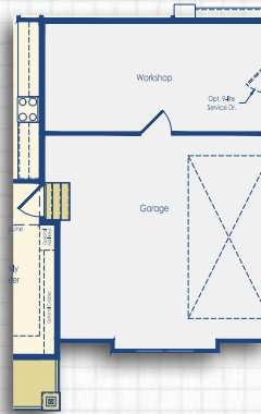
Optional Side Load Garage with 9' Garage Extension and Optional Workshop Craftsman Style
