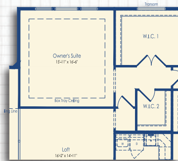
Optional Owner's Suite Entry
