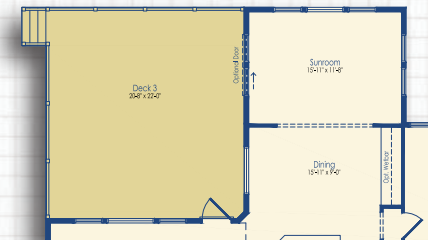
Optional Sunroom with Deck III
