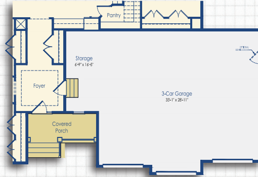
Optional 3-Car Front Load Garage with Optional 4' Extension Elevation D
