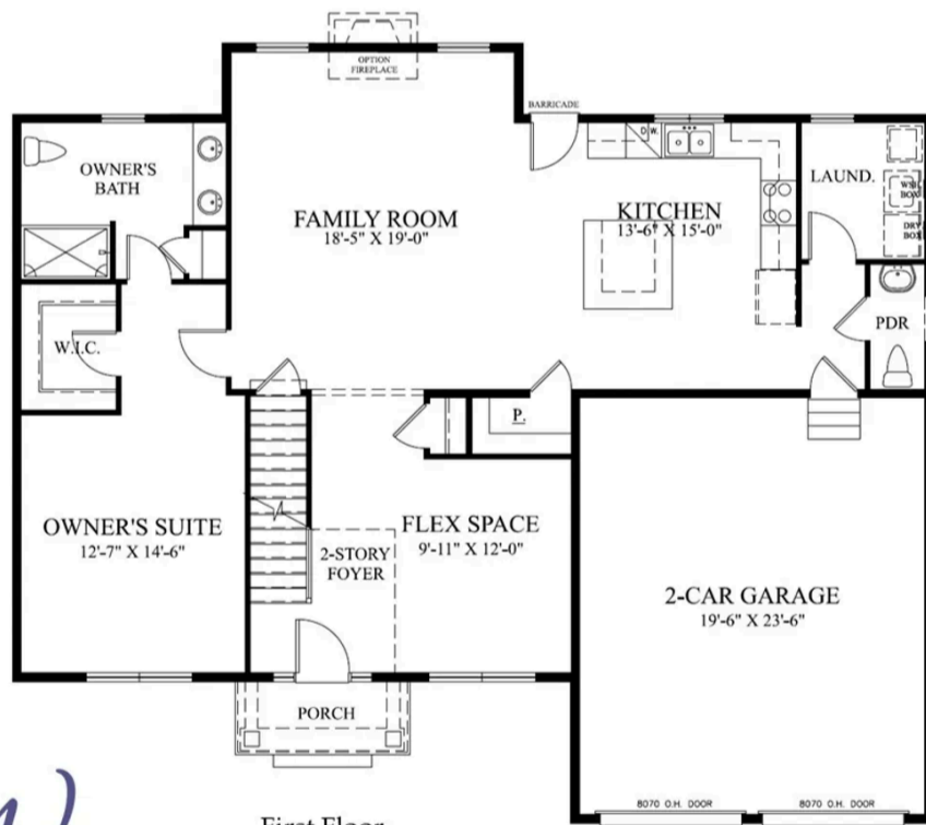
First Floor (Traditional Elevation)
