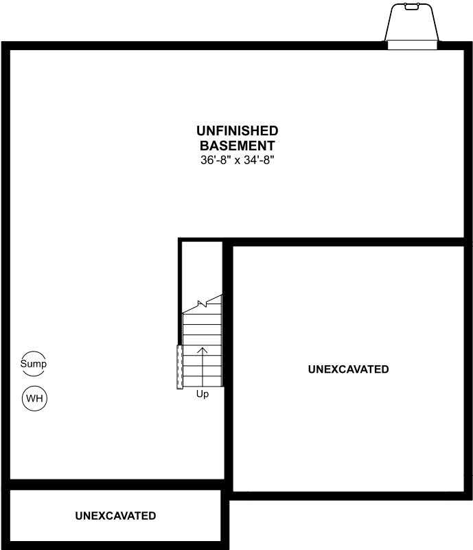
Basement
