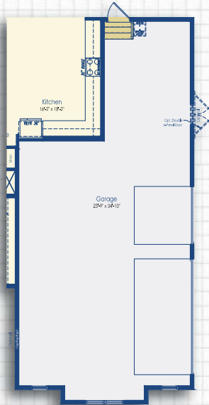
Optional 3-Car Side Load Garage Elevation B
