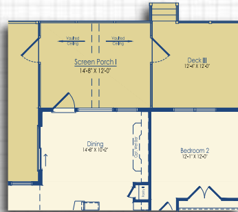
Optional Screen Porch I with Optional Deck III and Optional Deck IV
