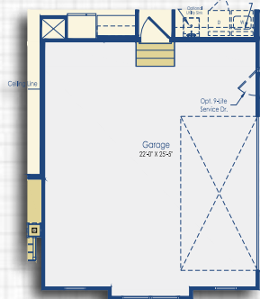
Optional Side-Load Garage with Optional 4' Extension Elevation C & D
