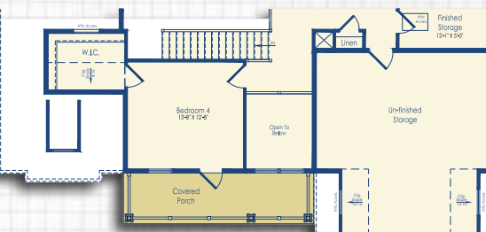
Optional Elevation C Second Floor
