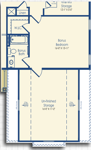
Optional Bonus Bedroom with Unfinished Storage and Optional 3-Car Side-Load Garage Elevation C
