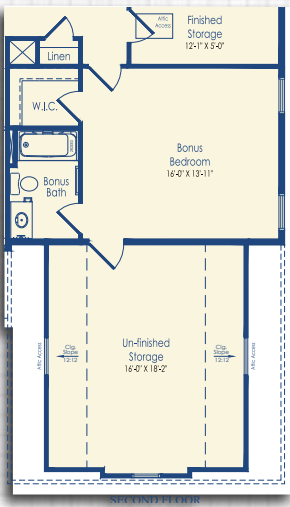
Optional Bonus Bedroom with Unfinished Storage and Optional 3-Car Side-Load Garage Elevation D
