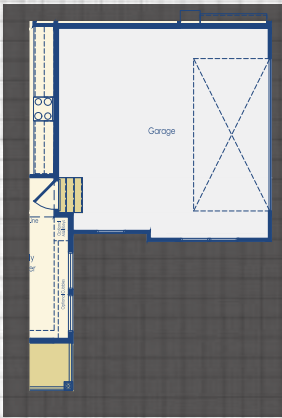
Optional Side Load Garage Schell Style C
