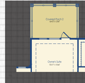
Optional Covered Porch II with Sunroom Below
