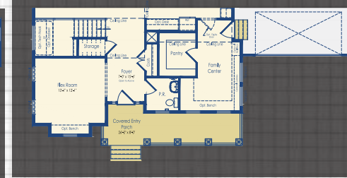
First Floor Optional Southern Style
