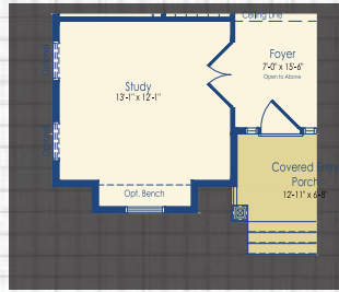
Optional Study Schell Style A, C, and Southern Style
