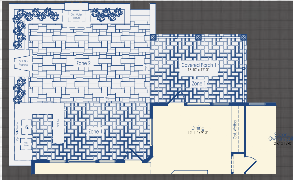
Optional Courtyard with Covered Porch I
