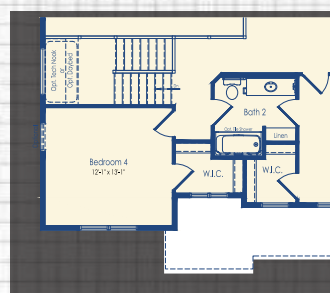
Optional Bedroom 4 Craftsman Style
