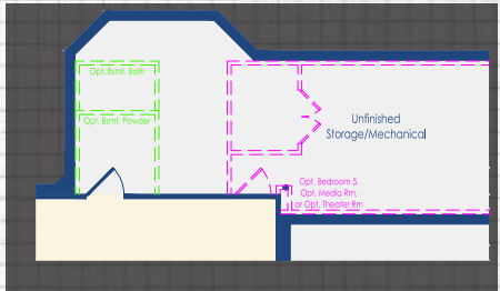
Optional Finished Basement with Dining Room Bay Window
