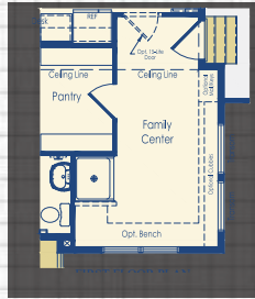
Optional Dog Wash in Family Center
