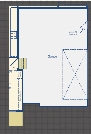
Optional Side Load with 9' Garage Extension Southern Style
