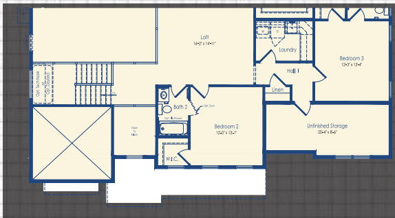
Second Floor with Optional 9' Garage Extension Schell Style C
