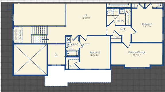
Second Floor with Optional 9' Garage Extension Craftsman Style
