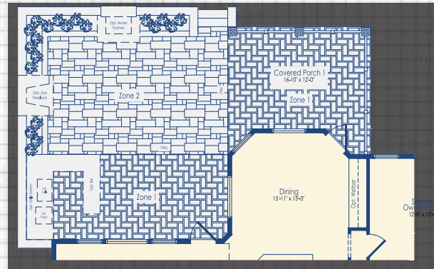
Optional Courtyard and Covered Porch with Dining Room Bay Window
