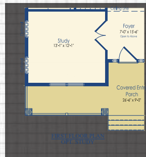
Optional Study Schell Style B
