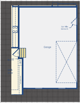
Optional Side Load with 9' Garage Extension Schell Style B
