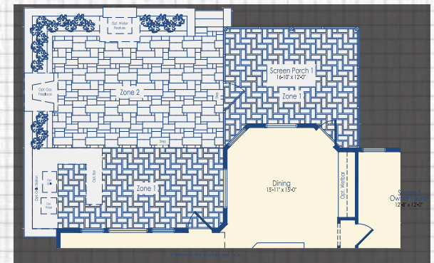
Optional Courtyard and Screen Porch I with Dining Room Bay Window
