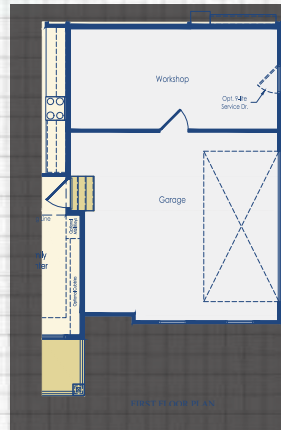
Optional Side Load Garage with 9' Garage Extension and Optional Workshop Southern Style
