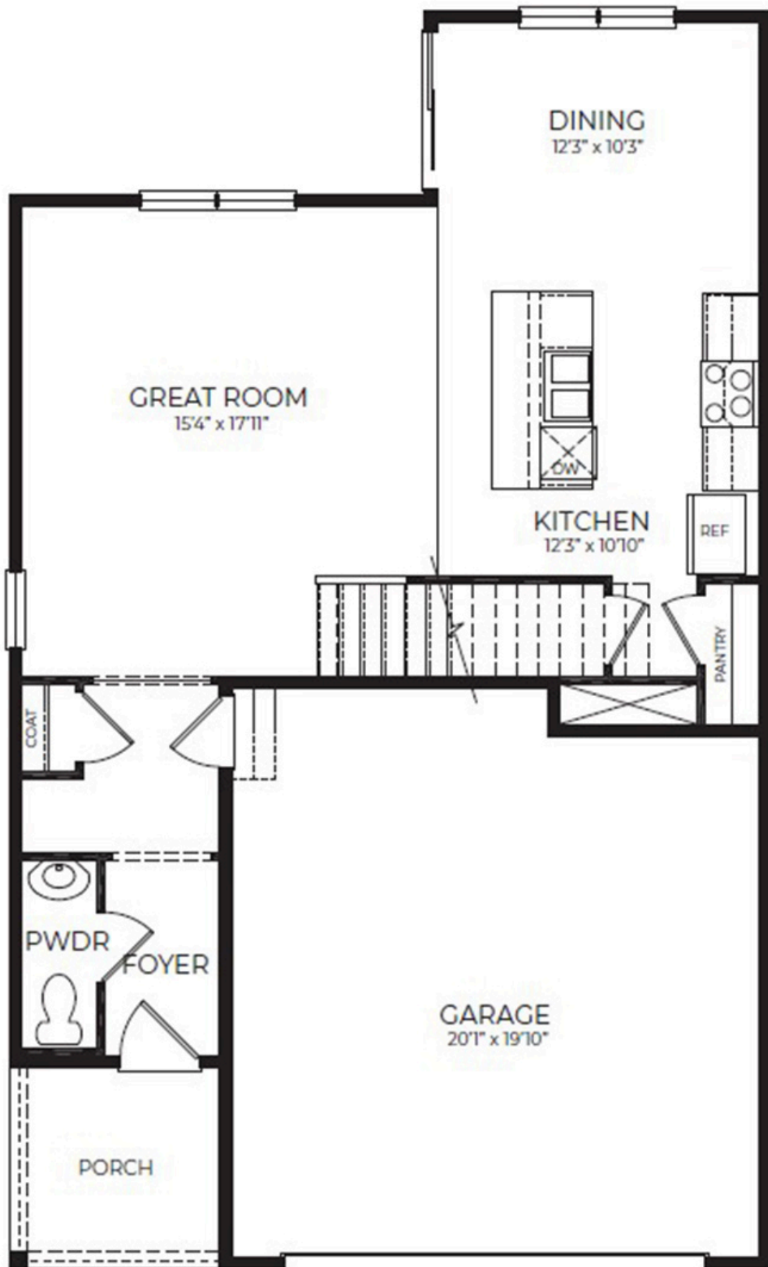
FIRST FLOOR
