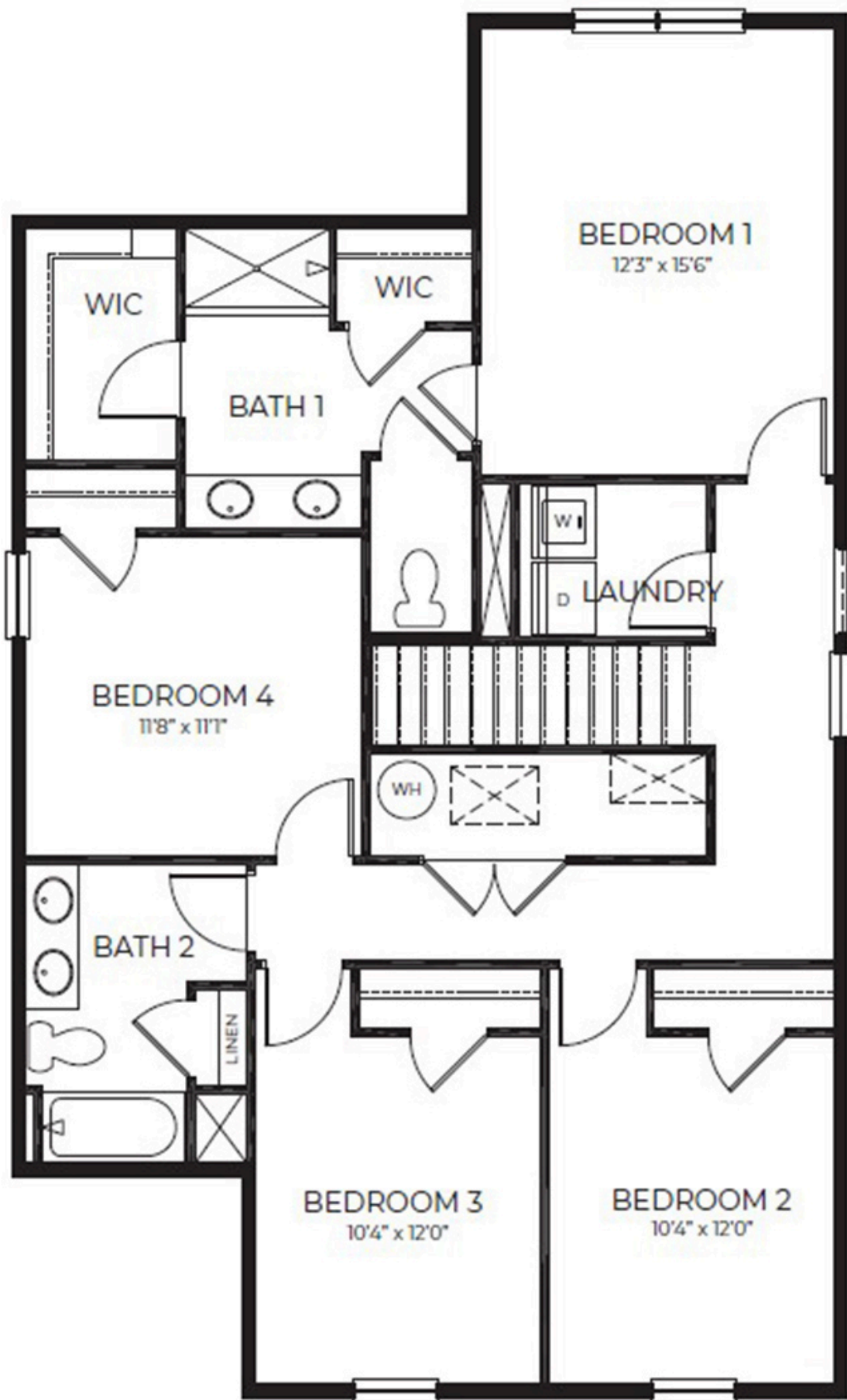
SECOND FLOOR
