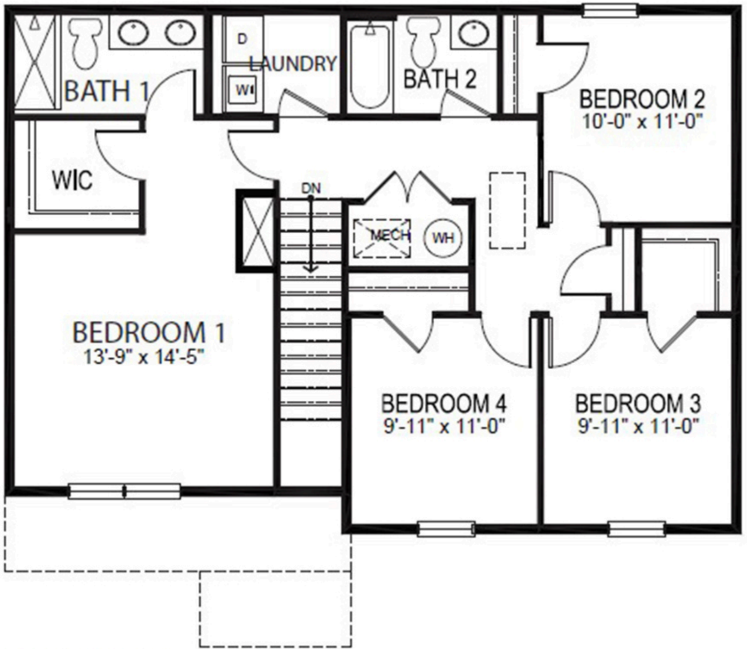
SECOND FLOOR
