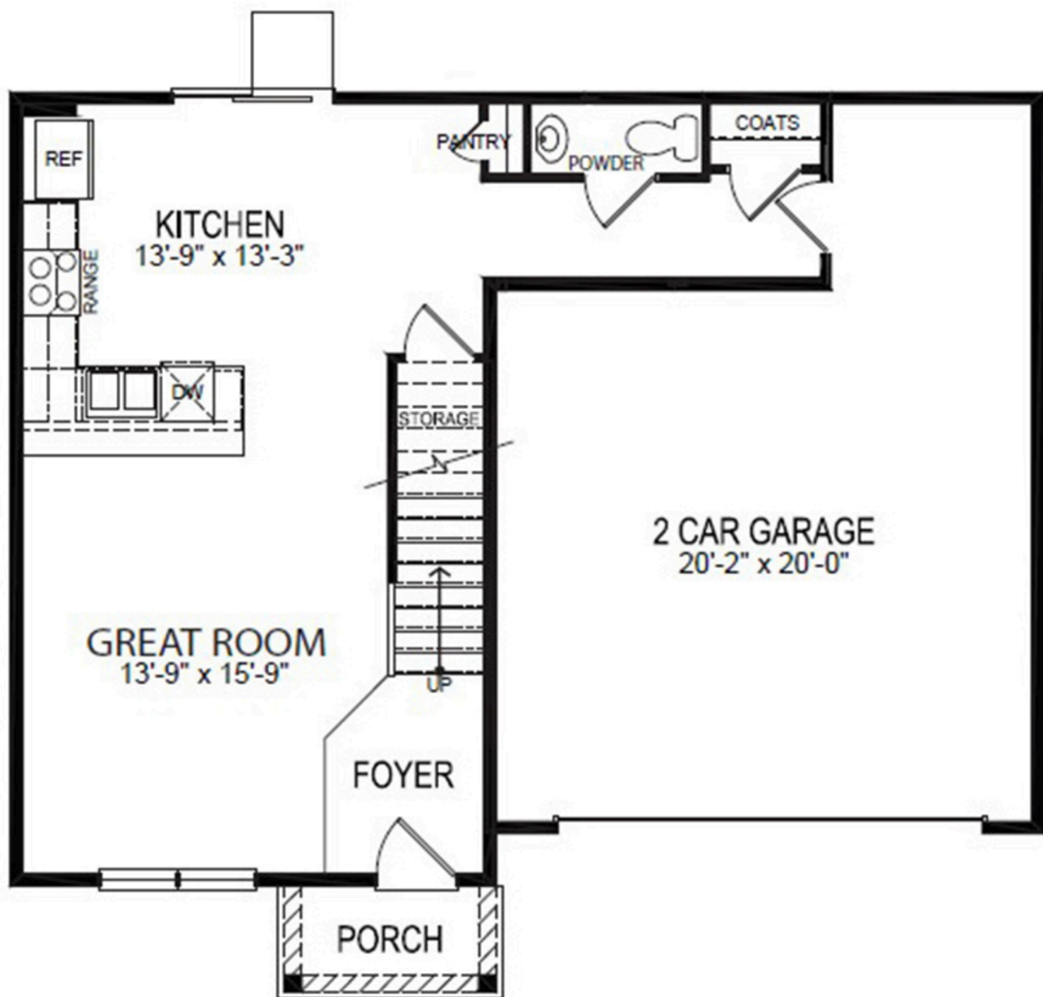
FIRST FLOOR
