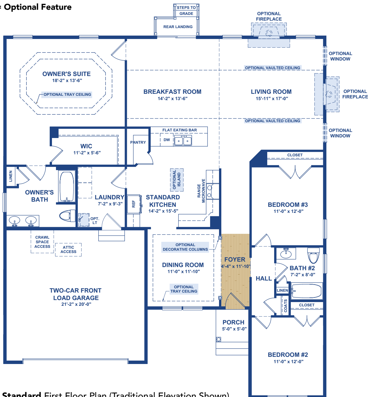
Standard First Floor Plan (Traditional Elevation Shown)
