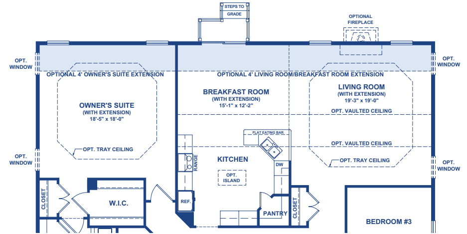
Optional 4' Rear Extension
