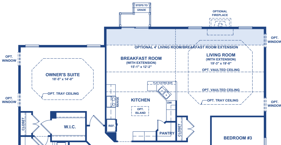
Optional 4' Living Room/Breakfast Room Extension
