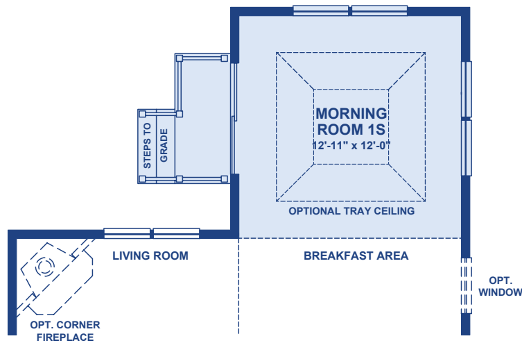
Optional Morning Room 1S
