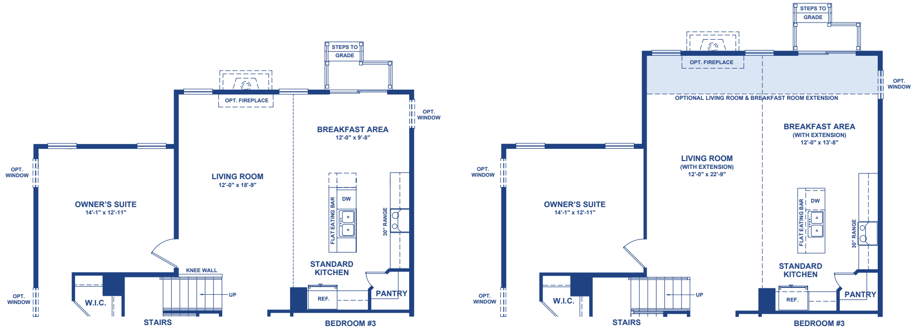
Standard First Floor Plan
