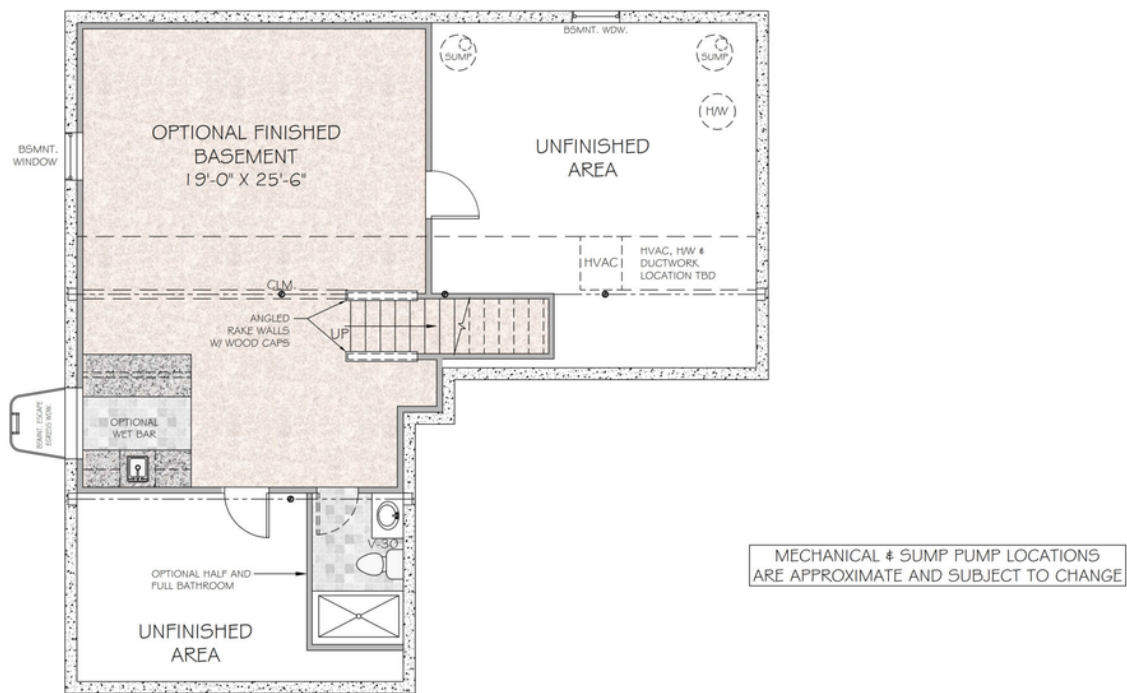
OPTIONAL FINISHED BASEMENT PLAN
