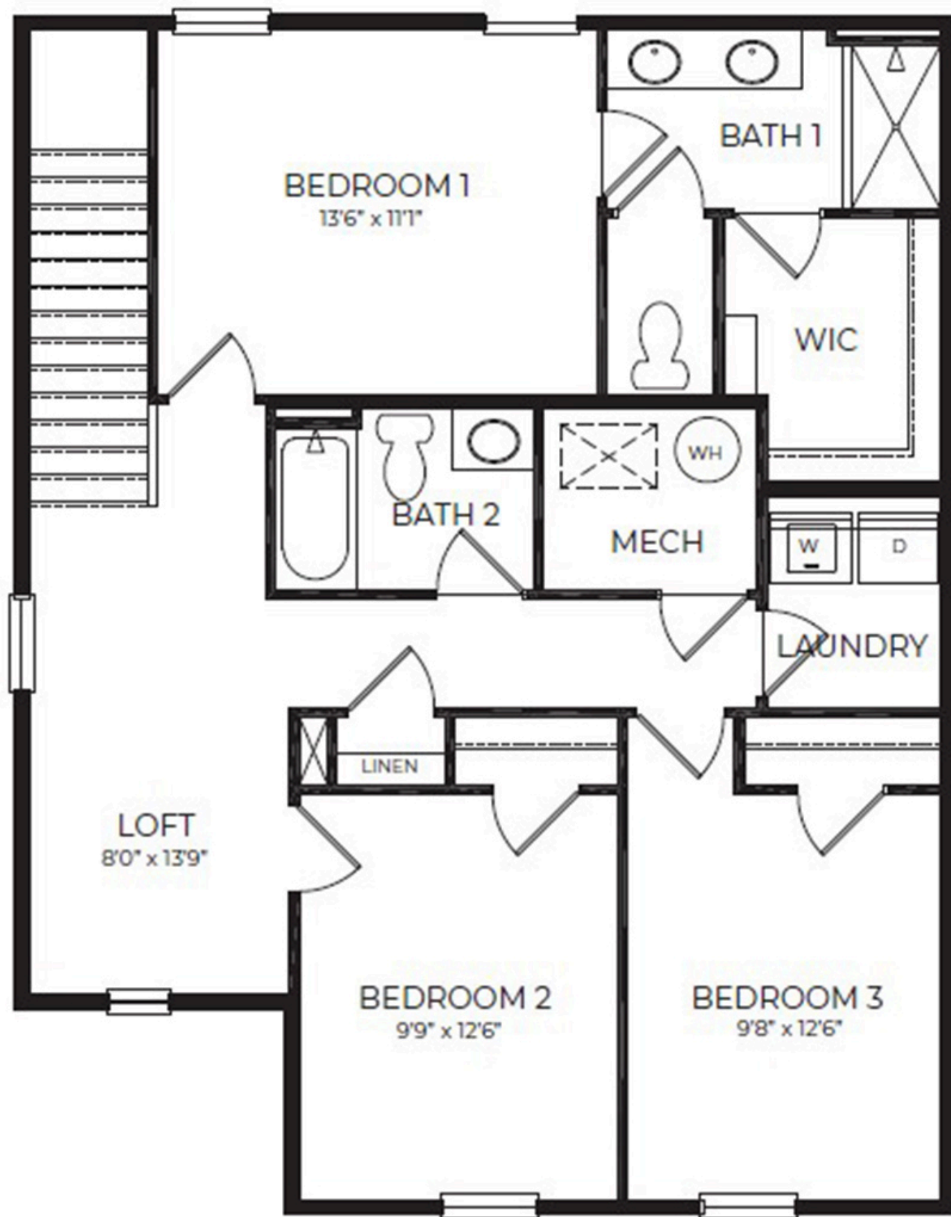
SECOND FLOOR
