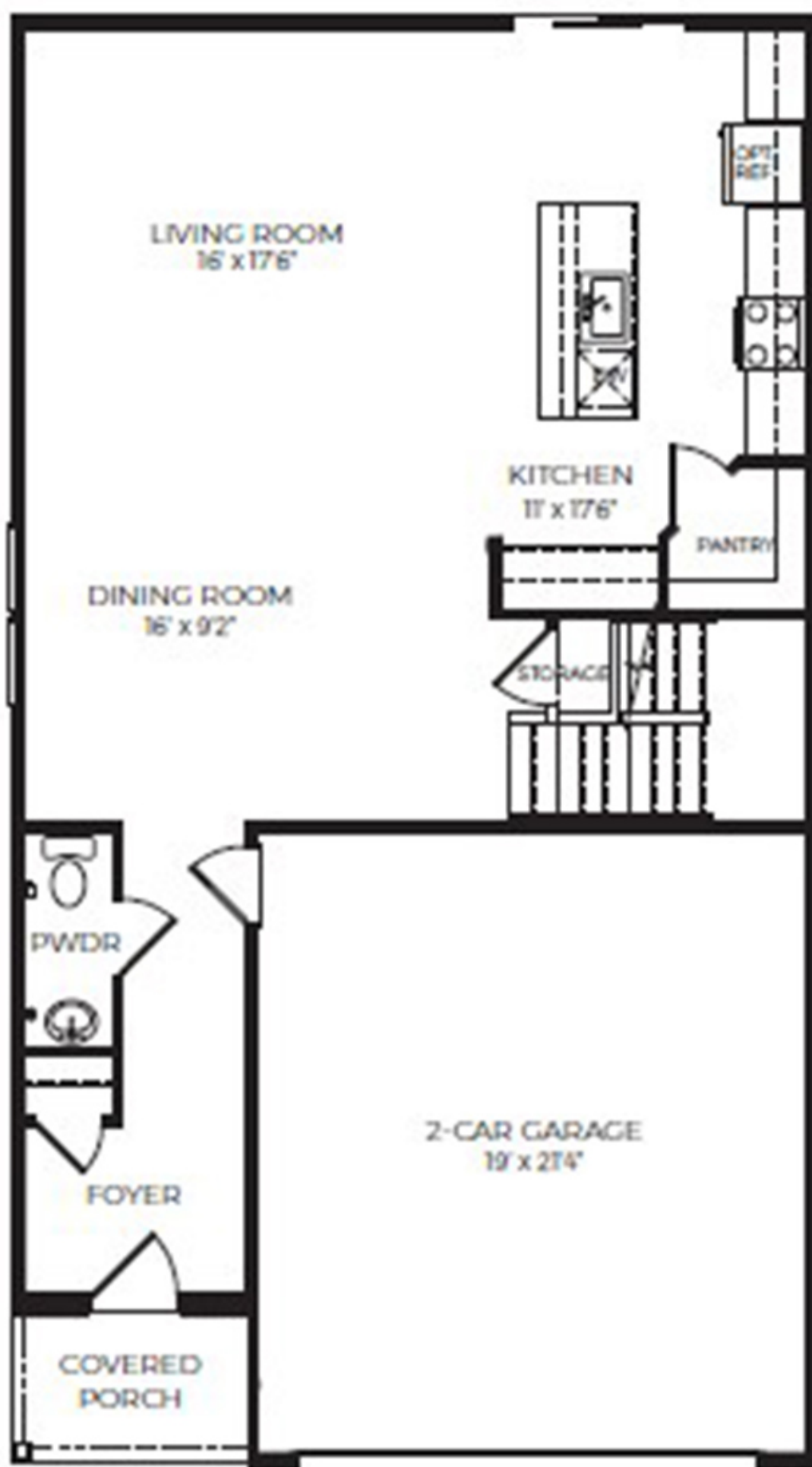
FIRST FLOOR
