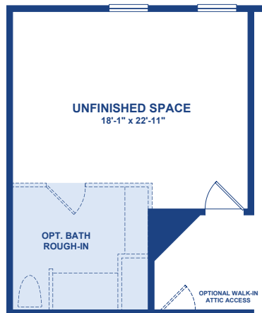
Optional Bath Rough-In 45003
