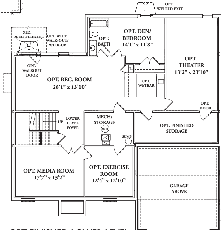
OPT. FINISHED LOWER LEVEL W/ OPT. IN-LAW SUITE
