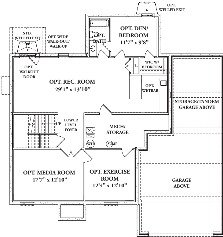
OPT. FINISHED LOWER LEVEL
