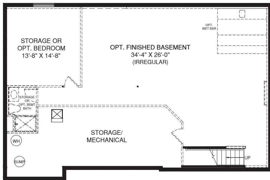
OPT. BEDROOM W/ OPT. BSMT. BATH
