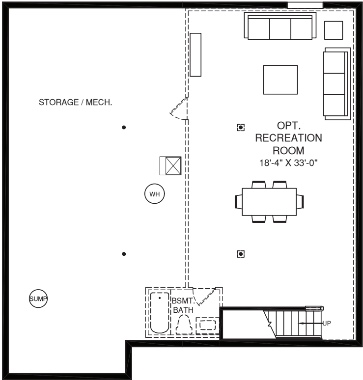
LOWER LEVEL
