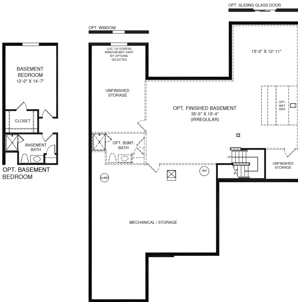
LOWER LEVEL
