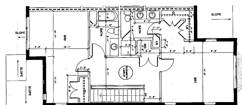
7 ELIZABETH LANE - SECOND FLOOR 1/4" = 1'-0"
