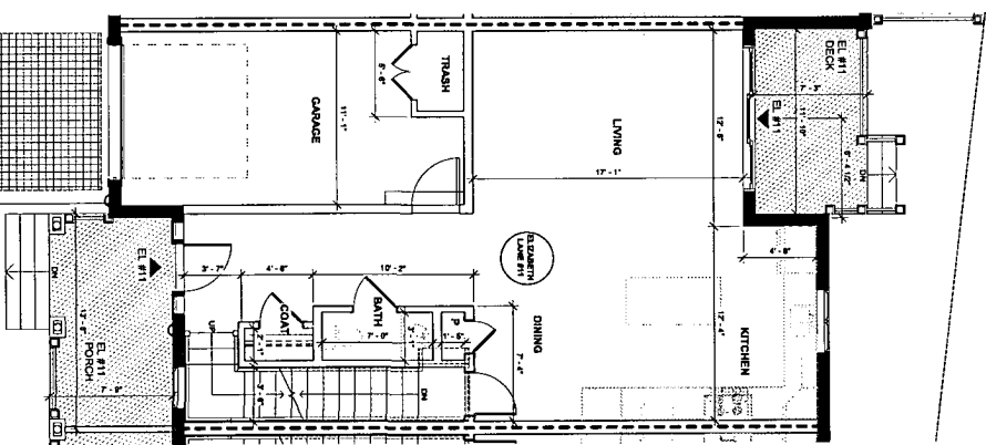
② 11 ELIZABETH LANE - FIRST FLOOR 1/4" = 1'-0"
