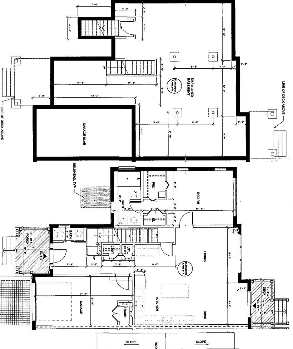
1 17 ELIZABETH LANE - BASEMENT
