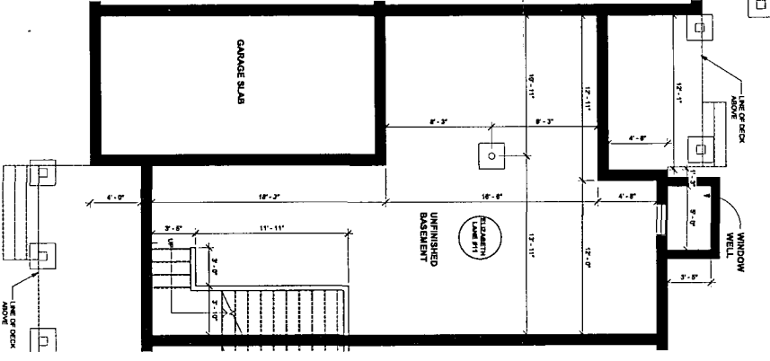
① 11 ELIZABETH LANE - BASEMENT 1/4" = 1'-0"
