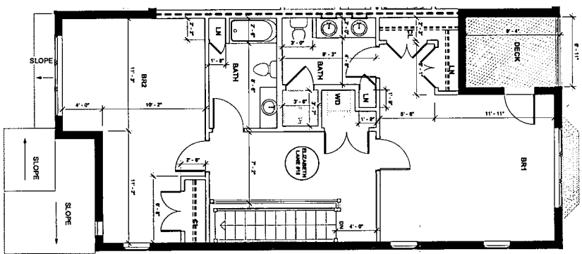
3 15 ELIZABETH LANE - SECOND FLOOR 1/4" = 1'-0"
