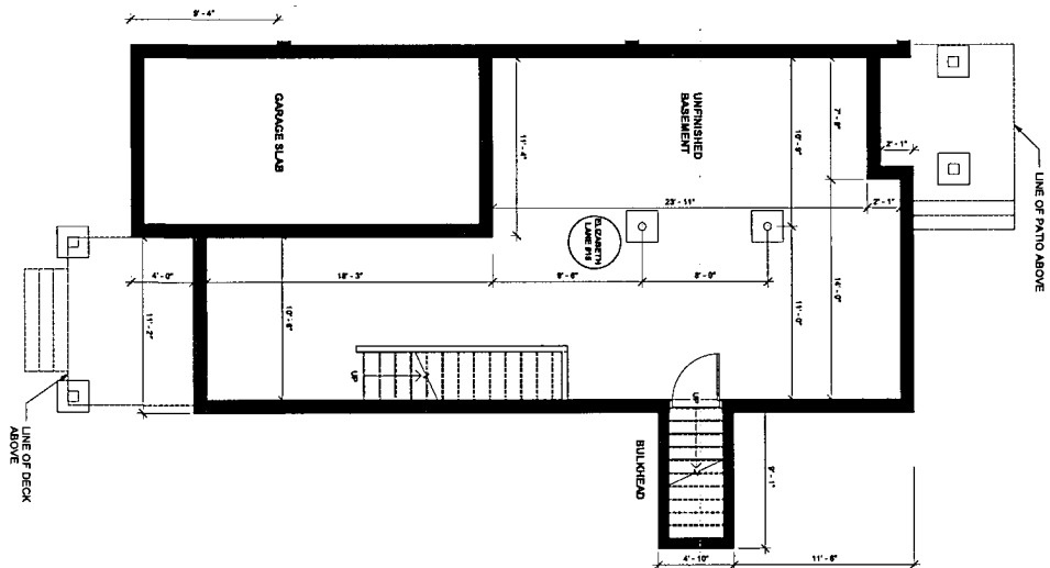
1 15 ELIZABETH LANE - BASEMENT 1/4" = 1'-0"
