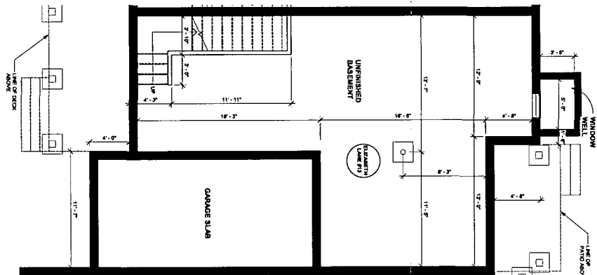
① 13 ELIZABETH LANE - BASEMENT 1/8" = 1'-0"
