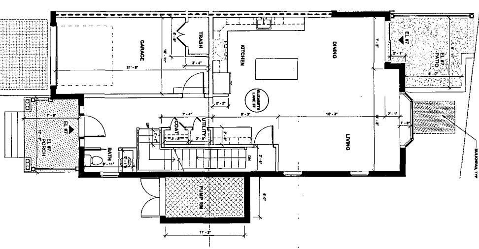
7 ELIZABETH LANE - FIRST FLOOR 1/4" = 1'-0"
