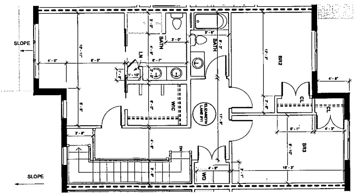
③ 11 ELIZABETH LANE - SECOND FLOOR 1/4" = 1'-0"
