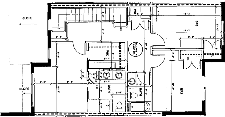
③ 13 ELIZABETH LANE - SECOND FLOOR 1/8" = 1'-0"
