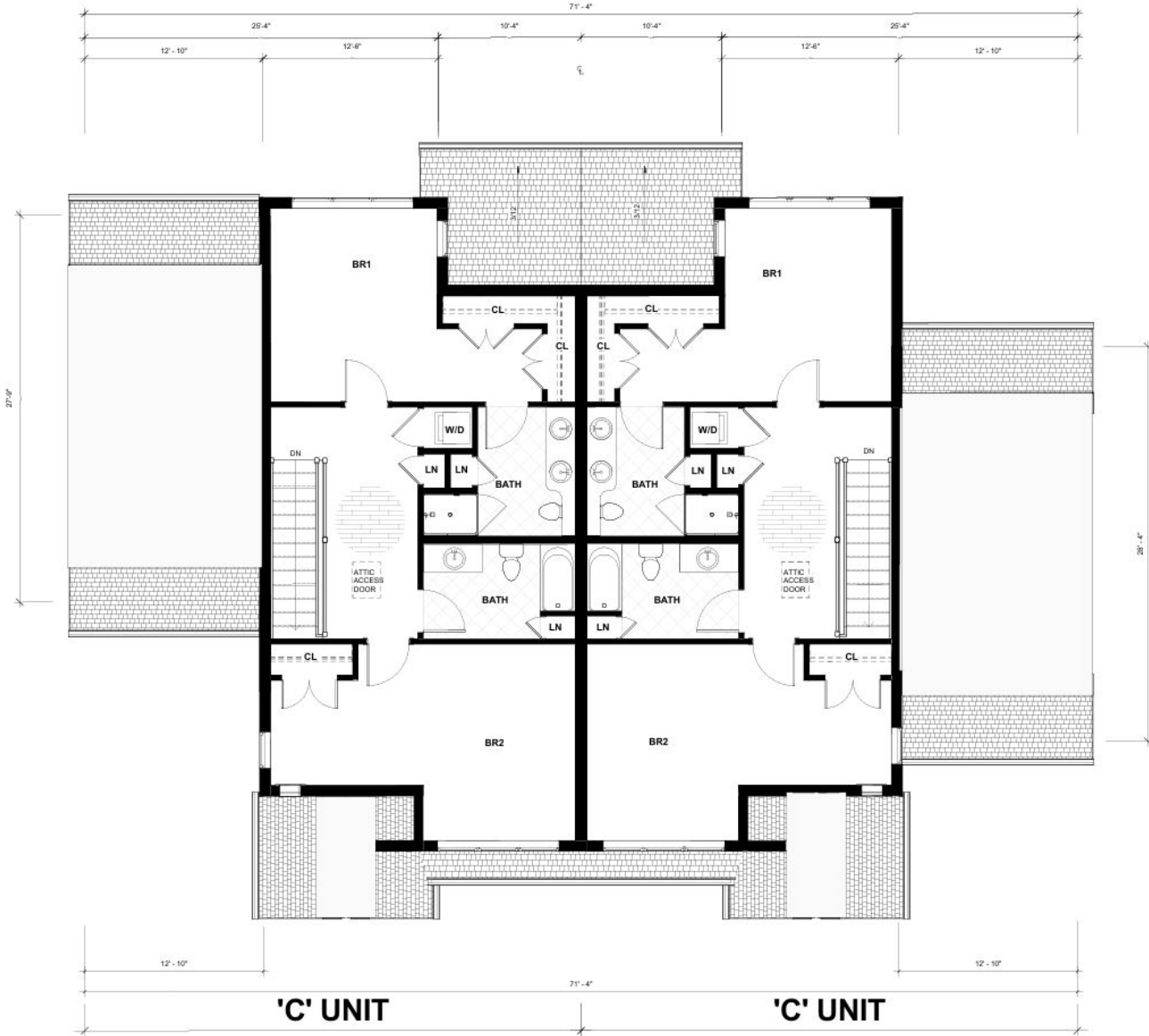
1 BLDG B-SECOND FLOOR PLAN 1/4" = 1'-0"
