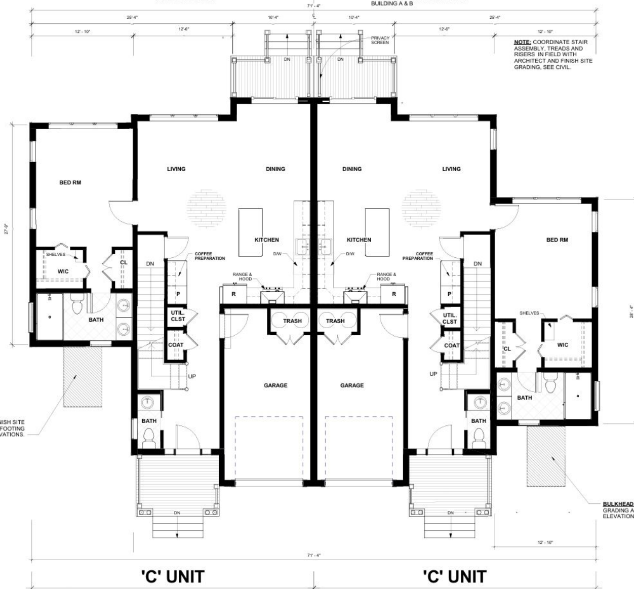
1 BLDG B- FIRST FLOOR PLAN 1/4" = 1'-0"
