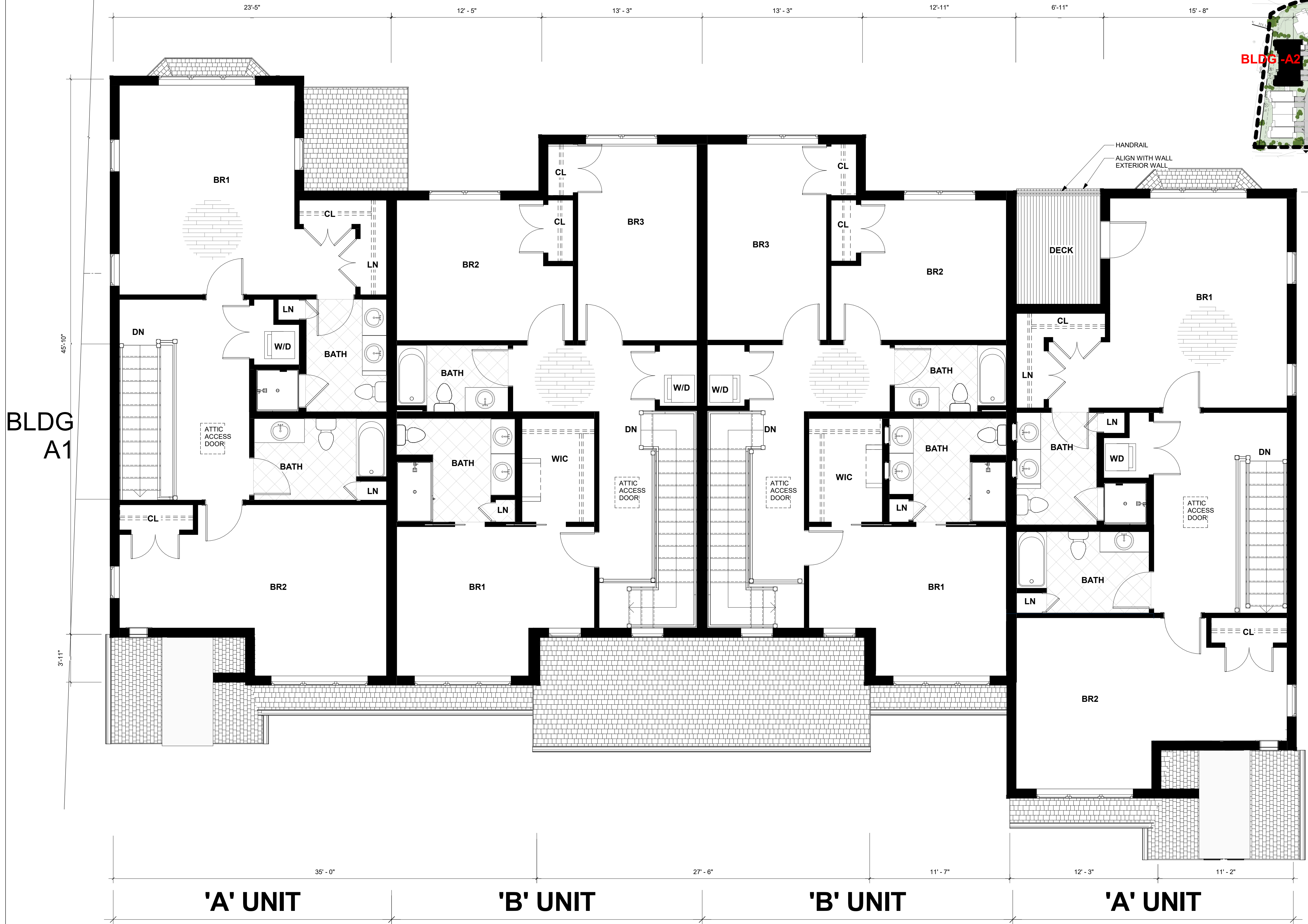
1 BLDG A2 -SECOND FLOOR PLAN 1/4" = 1'-0"
