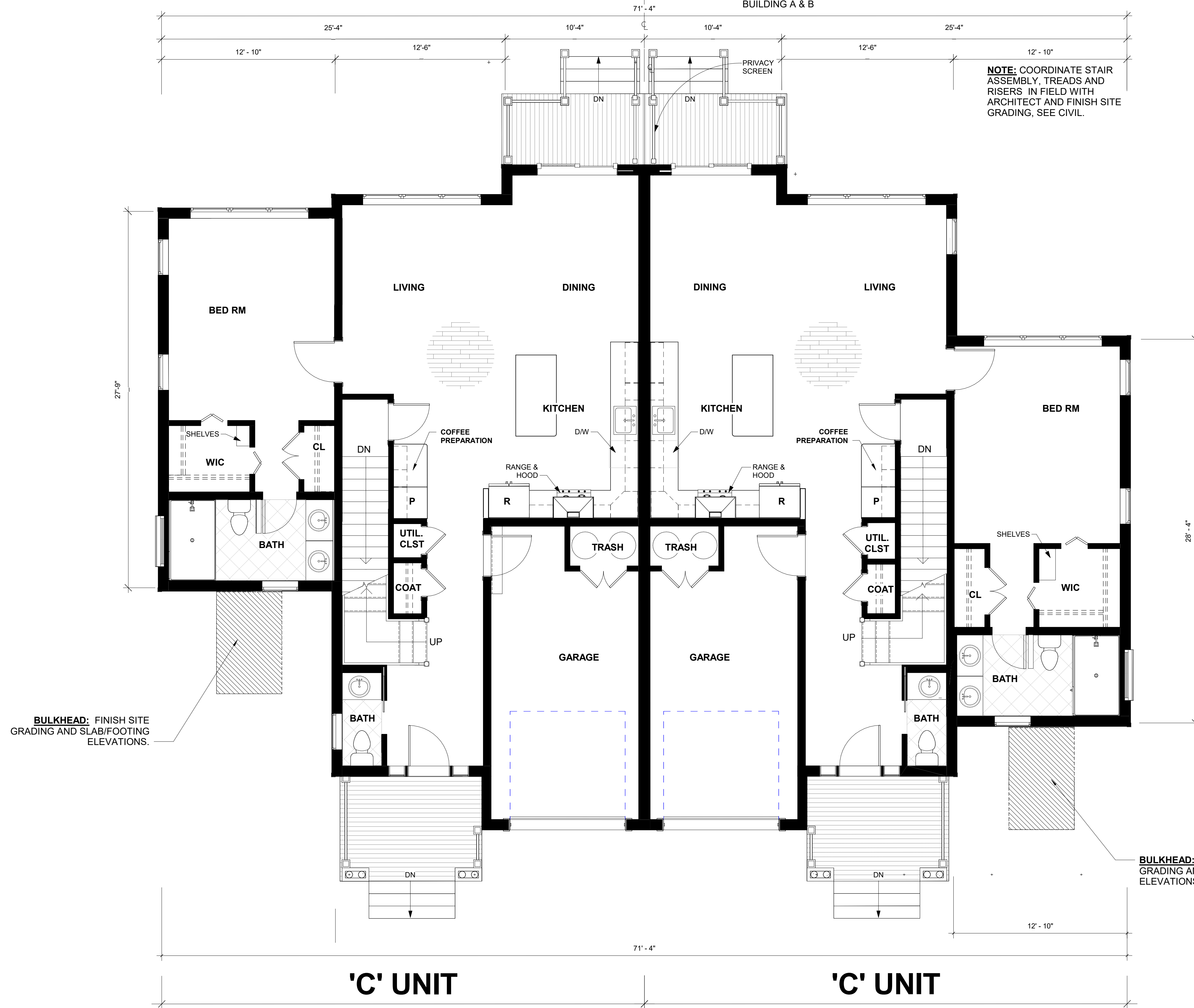
1 BLDG B- FIRST FLOOR PLAN 1/4" = 1'-0"
