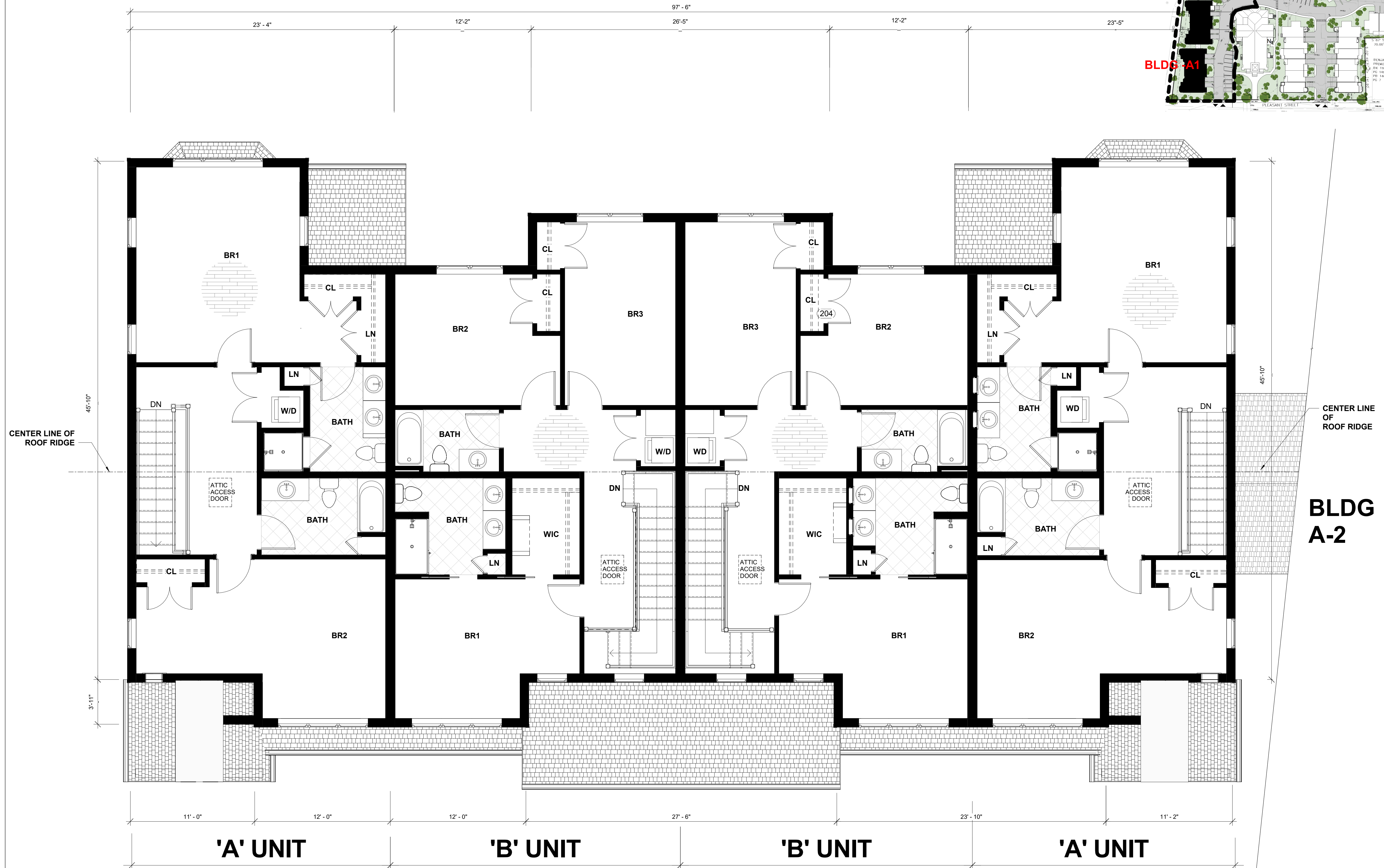
1 BLDG A1 -SECOND FLOOR PLAN 1/4" = 1'-0"
