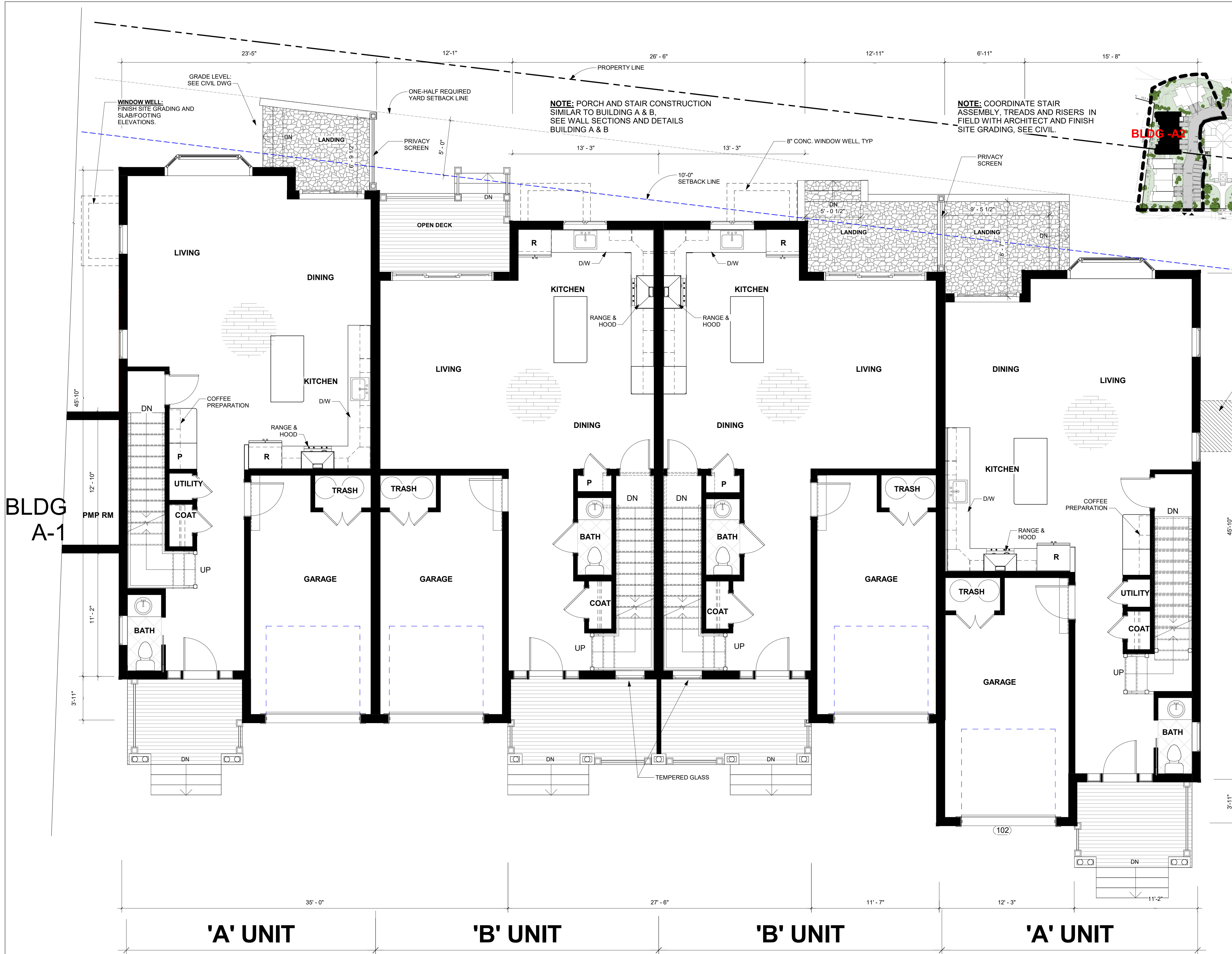
1 BLDG A2 - FIRST FLOOR PLAN 1/4" = 1'-0"
