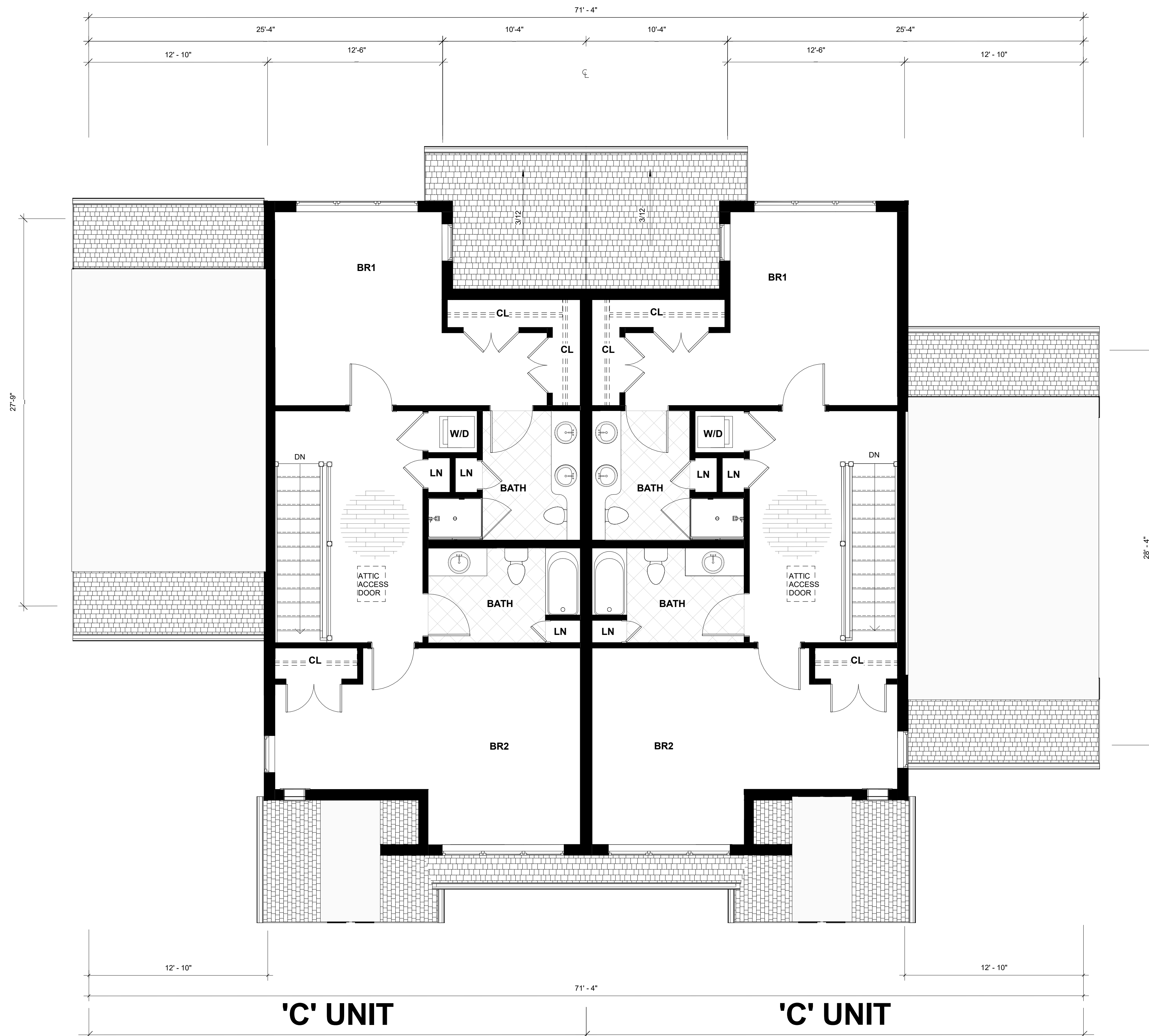
1 BLDG B-SECOND FLOOR PLAN 1/4" = 1'-0"
