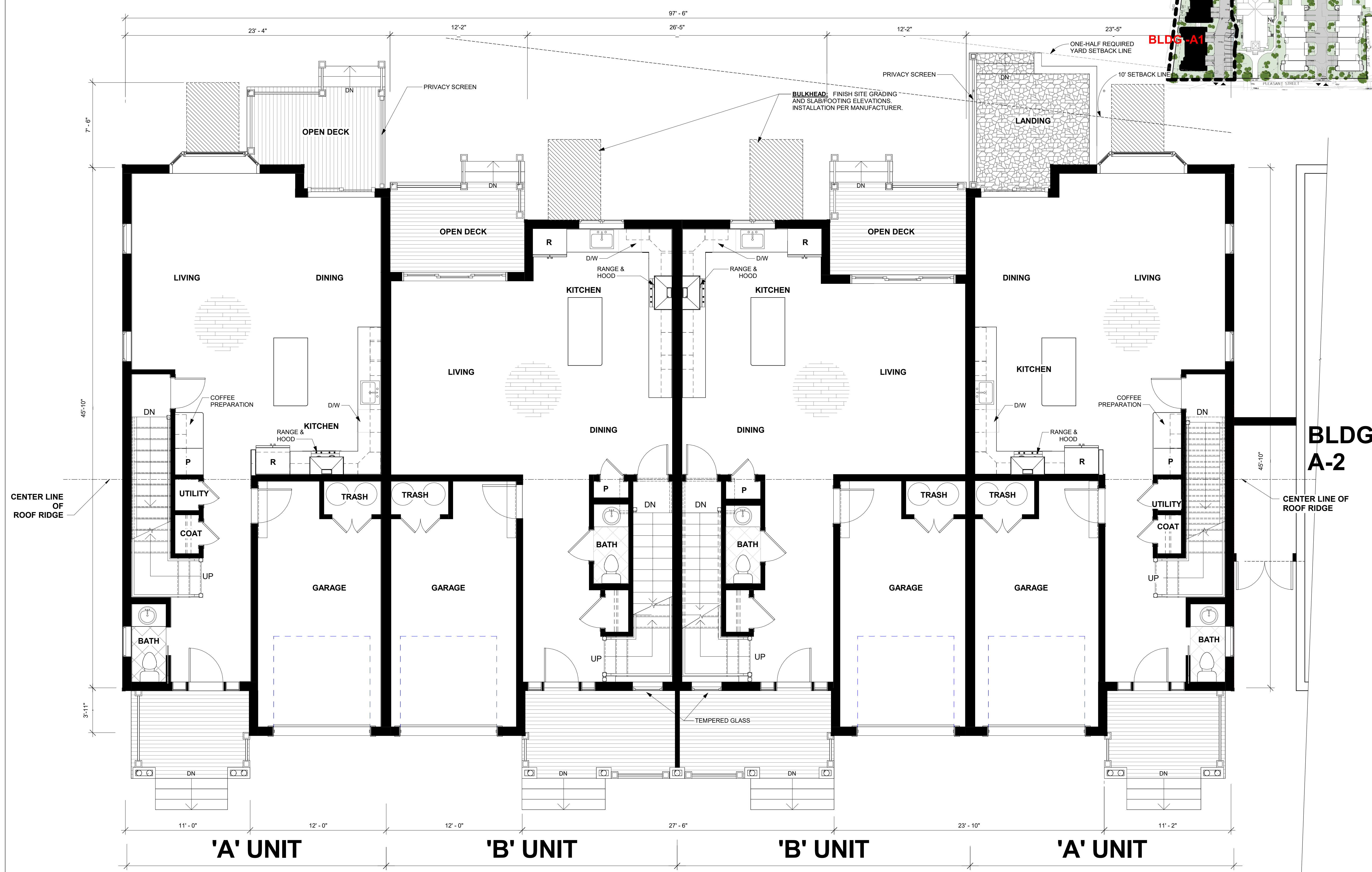
1 BLDG A1 - FIRST FLOOR PLAN 1/4" = 1'-0"
